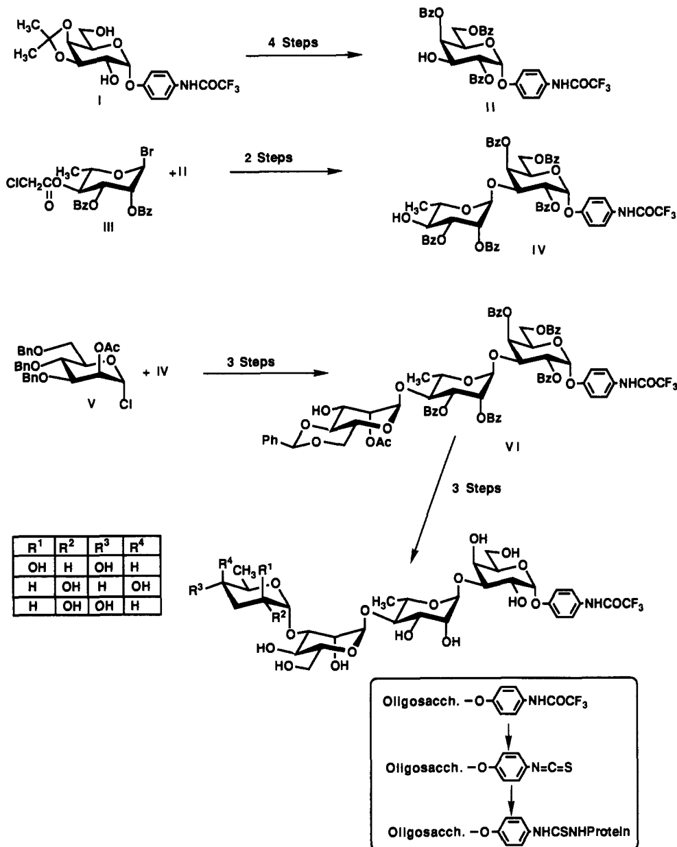
Figure 8. Syntheses of the Salmonella serogroups A, B, and D 1 tetrasaccharides.
